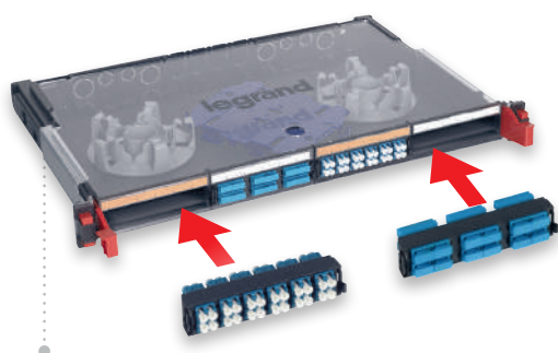
Modular panels
